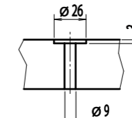
Z-Z (4 locations)
